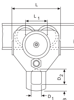
Model HTG 10.000 kg
