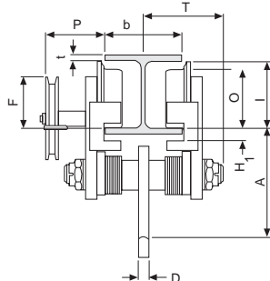
Model HTG 10.000 kg
